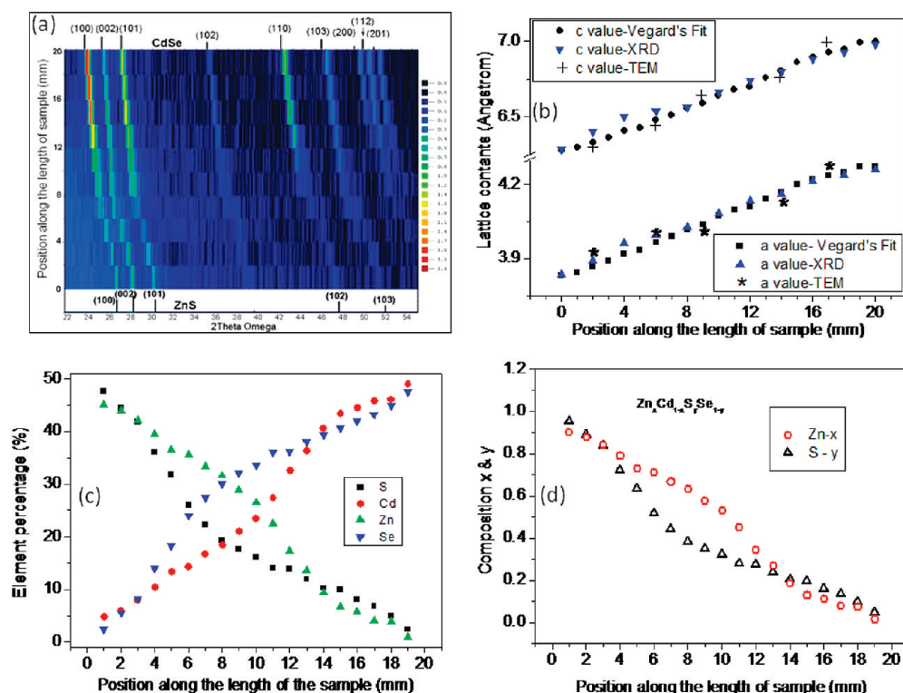
Figure 3. (a) Spatial XRD scan along the length of the 1D composition-graded sample with a step of 2 mm, as well as the standard 2\theta values for ZnS and CdSe wurtzite single crystals. (b) Position-dependent lattice constants a and c , along the length of the sample obtained from the fitting of XRD data (blue triangles), the Vegard law approximation (dark filled circles and rectangles), and the TEM measurements (crosses and stars). (c) Element profiles along the length of the 1D graded sample, (d) the corresponding converted position-dependent composition x and y .
